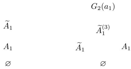
FIGURE 5. G_2 for p = 2 (left) and p = 3 (right)
