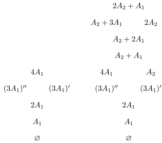
FIGURE 2. E_7 for p = 2 (left) and p = 3 (right)
