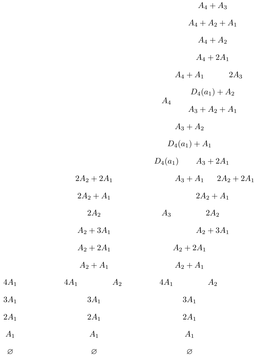
FIGURE 3. E_8 for p = 2 (left), p = 3 , (center), and p = 5 (right)
