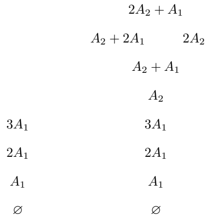
FIGURE 1. E_6 for p = 2 (left) and p = 3 (right)
