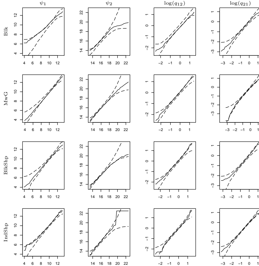
Figure 4: QQ plots for algorithms Blk, MwG, BlkShp, and IndShp, on D2 (Replicate 1). Dashed lines are approximate 95% confidence limits obtained by repeated sampling from iterations 1000 to 100 000 of a Gibbs sampler run; sample sizes were 10 000/ACT, which is the effective sample size of the data being compared to the Gibbs run.
